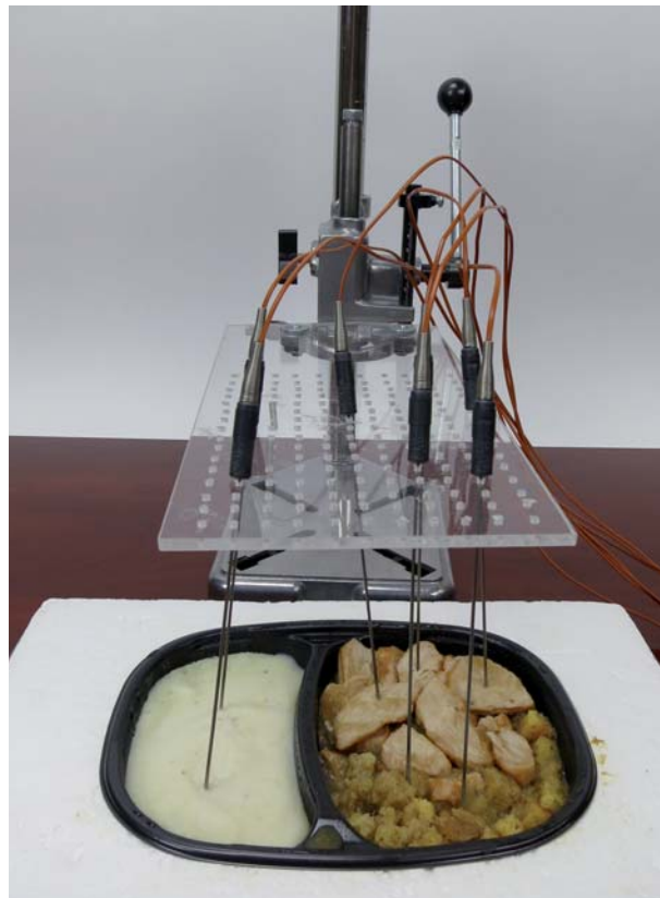
Figure 1. A "Hedgehog" thermocouple array with the thermocouples placed within food components. Tray of NRTE product is placed into the rigid foam tray holder to reduce heat loss during temperature measurement. The thermocouples may be raised or lowered with the large handle.
